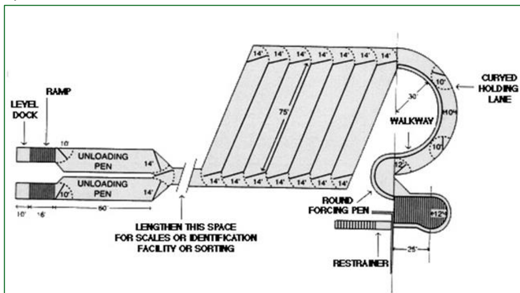
Temple Grandin's design showing oblong pens. This design was made for a cattle slaughterhouse but the left part (unloading and lairage pens) can also be applied to pig slaughterhouses.
